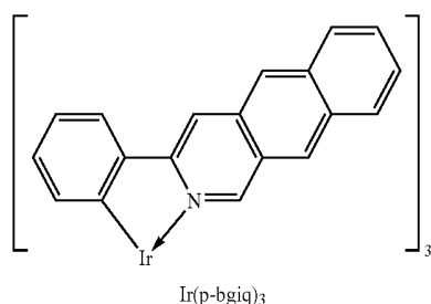
\text{Ir}(\text{p-bgiq})_3
